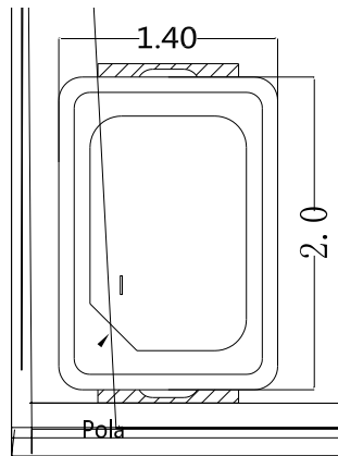
Fig.1-1 Top View
