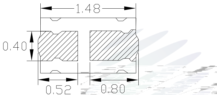
Fig.1-3 Bottom View
