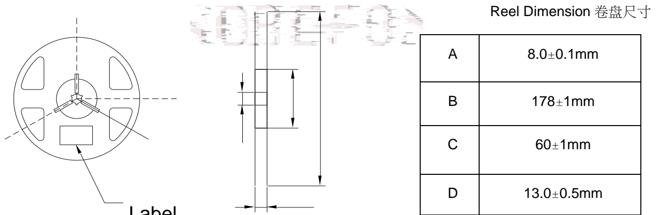
Fig.2-2 Reel Dimension 卷盘尺寸
