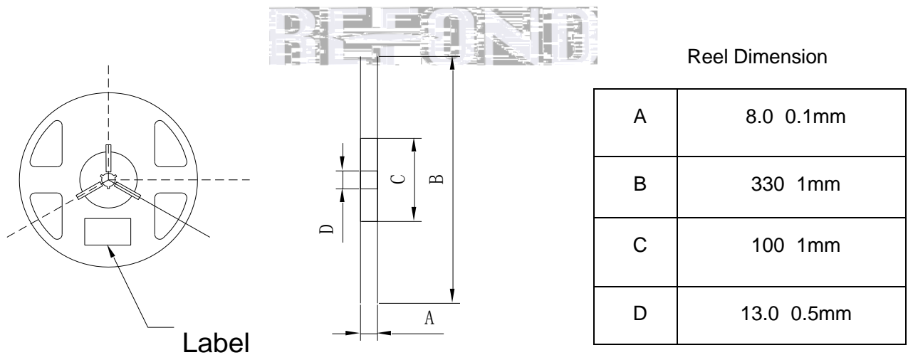
Fig.2-2 Reel Dimension
