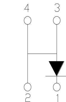
Fig.1-4 Polarity
