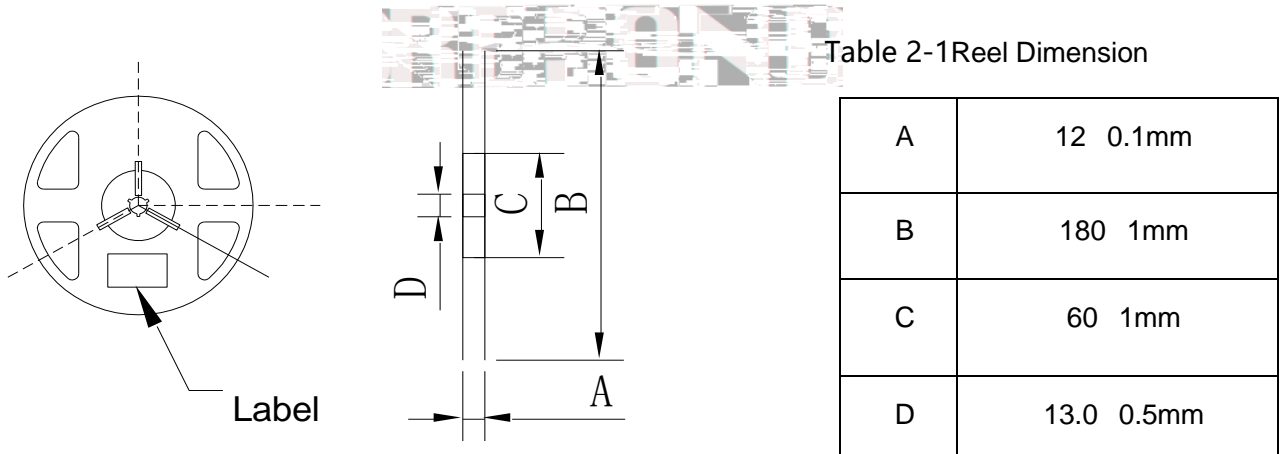
Fig.2-2 Reel Dimension
