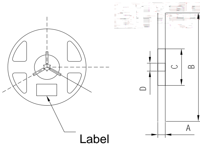
Fig.2-2 Reel Dimension 卷盘
