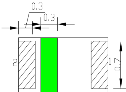
Fig.1-3 Bottom view
