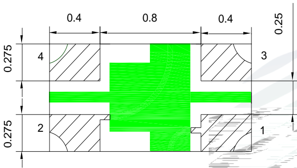
Fig.1-3 Bottom view
