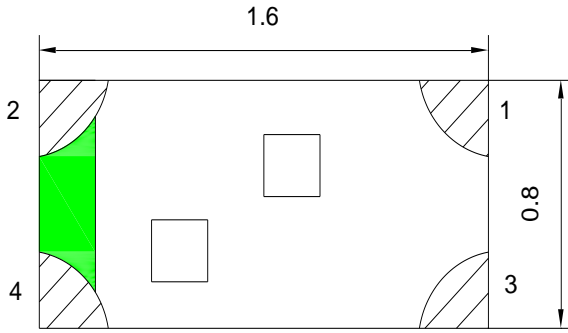
Fig.1-1 Top view
