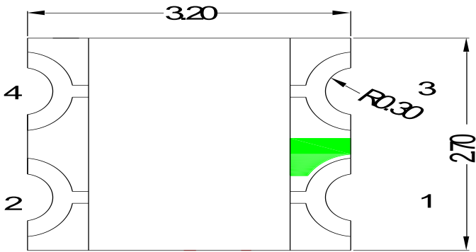
Fig.1-1 Top view
