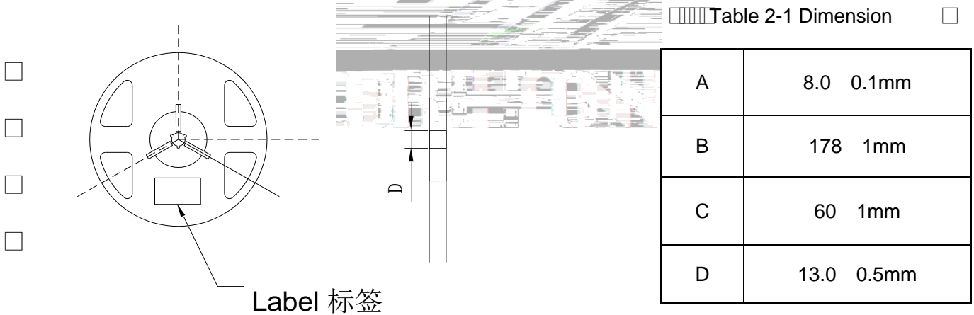
Fig.2-2 Reel Dimension 却
