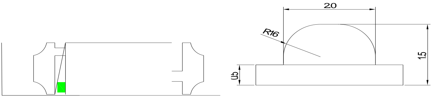
Fig.1-1 Top view
