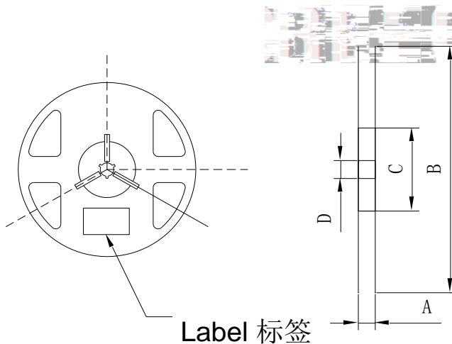
Fig.2-2 Reel Dimension
