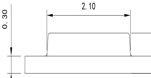
Fig.1-3 Side view 侧面视图
