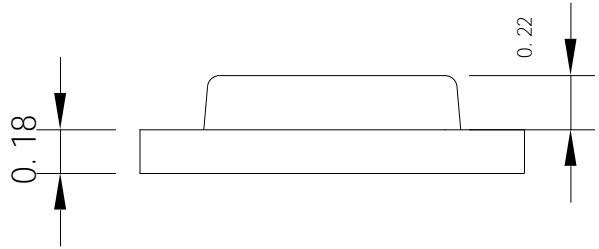
Fig.1-2 Side view
