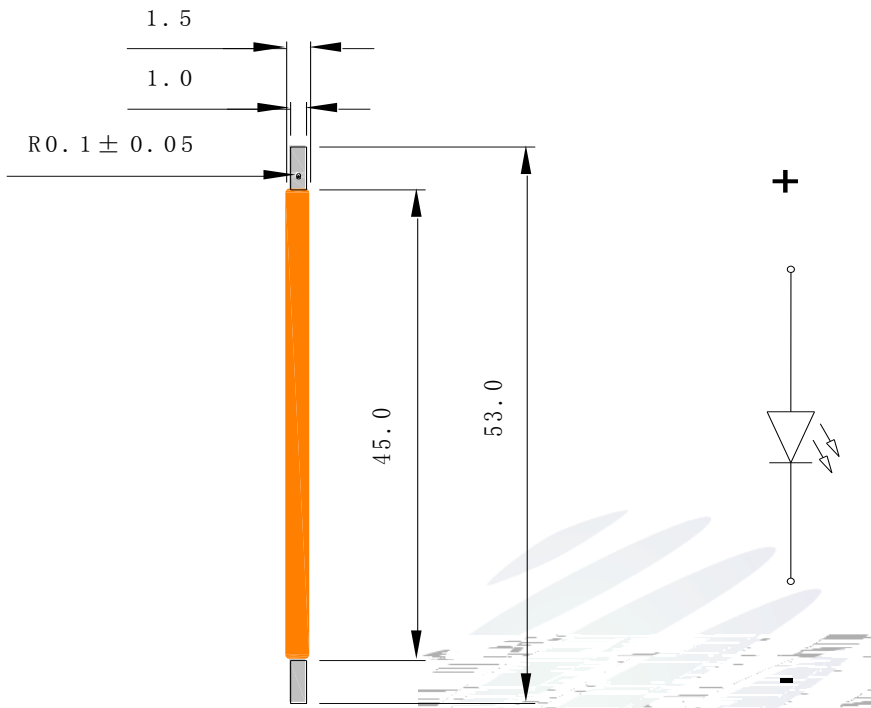
Fig.1-1 Top View
