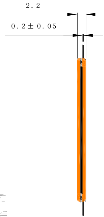
Fig.1-2 Side View
