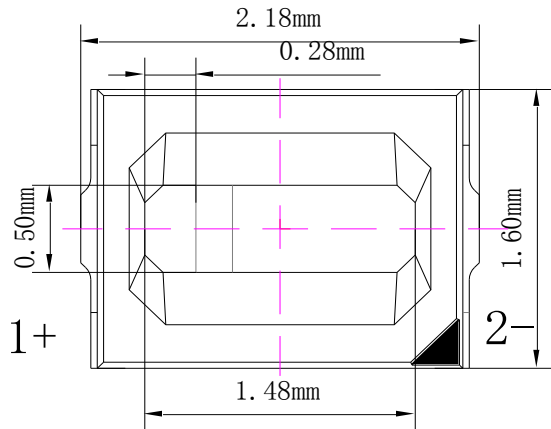
Fig.1-1 Top view
