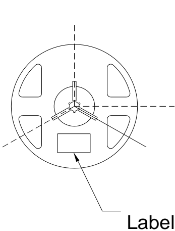
Fig.2-2 Reel Dimension
