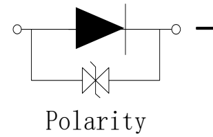
Fig.1-4 Polarity
