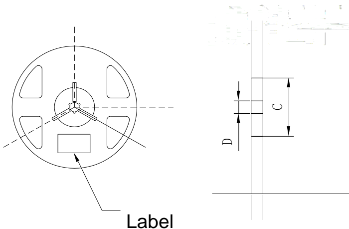
Fig.2-2 Reel Dimension
