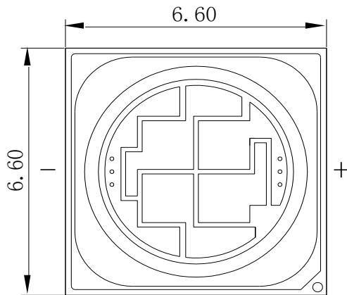
Fig.1-1 Top view
