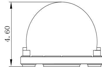
Fig.1-2 Side view
