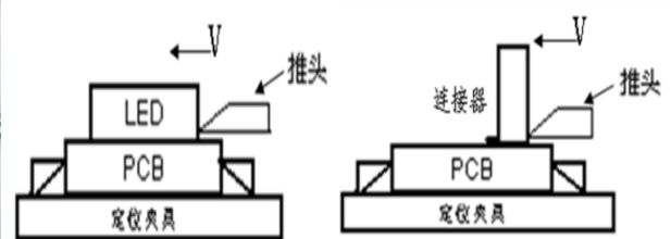
Fig 7-2 Push & Pull Test Method
