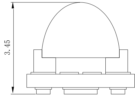
Fig.1-2 Side view
