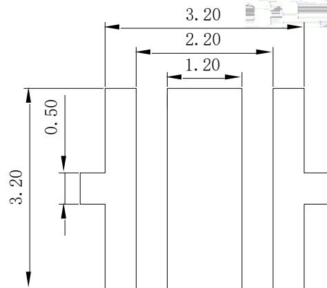
Fig.1-5 Soldering patterns
