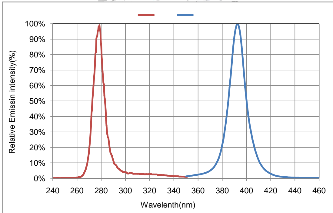
Fig.4-Spectrum Distribution
