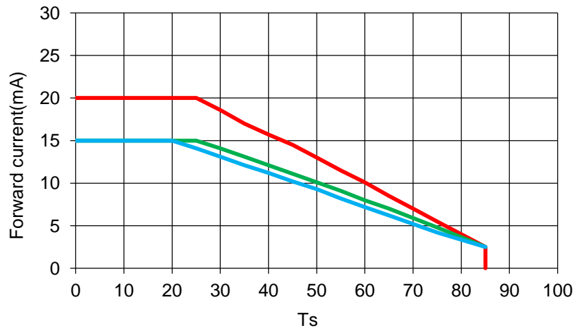
Fig 1-9 Solder Temperature Vs Forward Current
