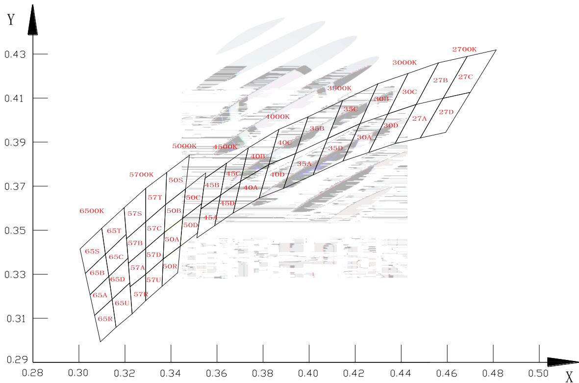
Fig.1-7 Chromaticity Coordinates
