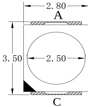
Fig.1-1 Top View
