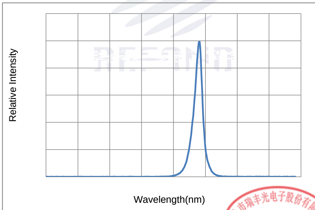
Fig. 1-14 Spectrum Distribution
