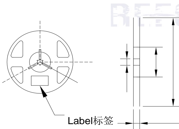
Fig.2-2 Reel Dimension
