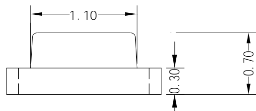
Fig.1-2 Side view
