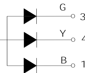
Fig.1-4 Polarity
