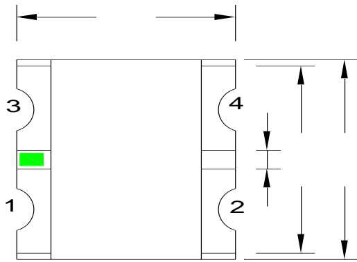
Fig.1-1 Top view
