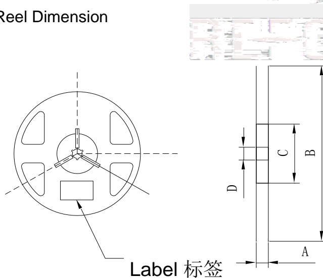
Fig.2-2 Reel Dimension
