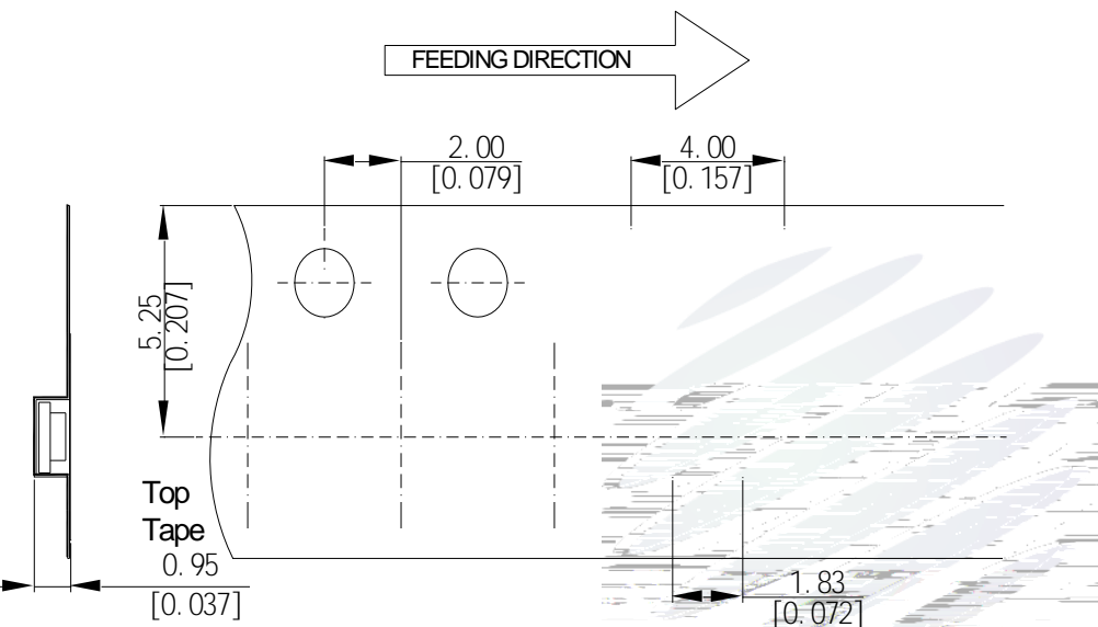
Fig.2-1 Carrier Tape Dimension
