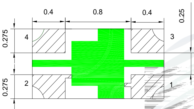
Fig.1-3 Bottom view
