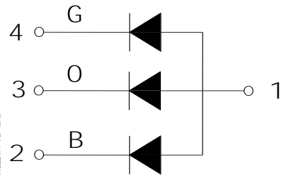
Fig.1-4 Polarity
