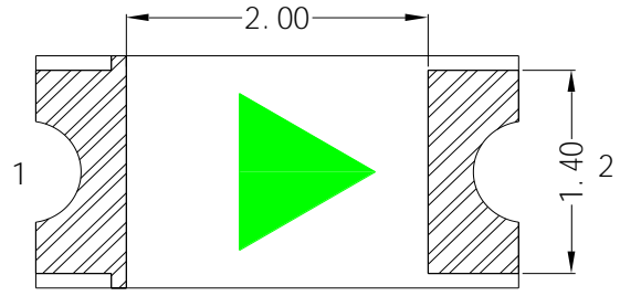
Fig.1-2 Bottom view
