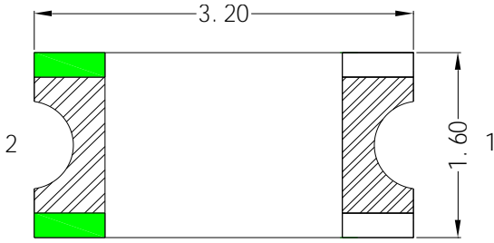
Fig.1-1 Top view
