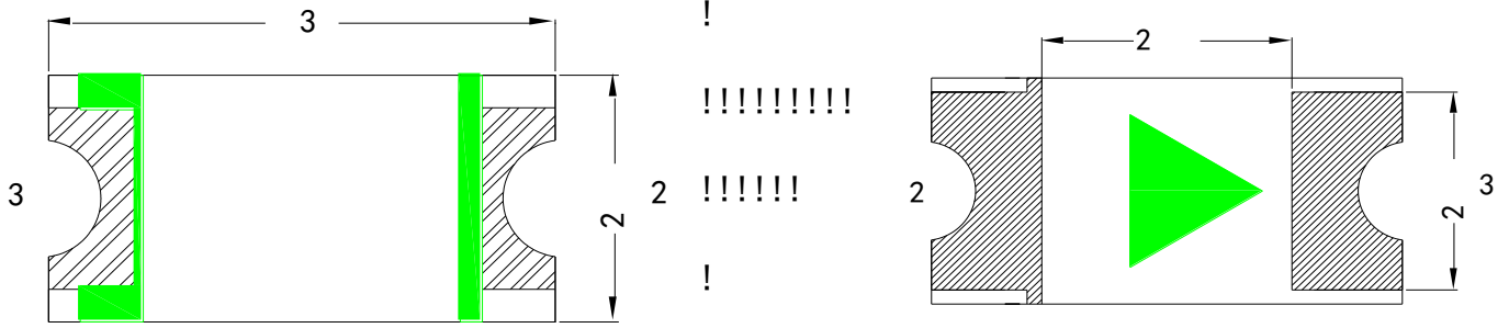
Fig.1-1 Top view!
