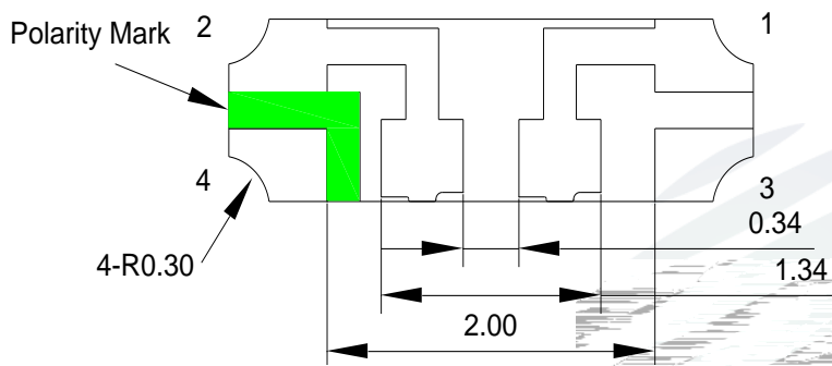
Fig.1-1 Top view
