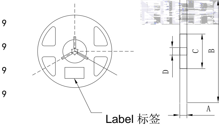
Fig.2-2 Reel Dimension 9
