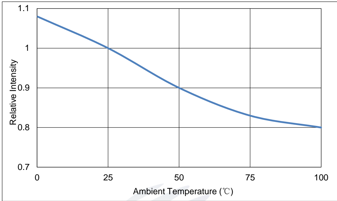
Fig 1-9 Pin Temperature Vs Relative Intensity 丙射
