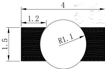
Fig.1-5 Soldering patterns
