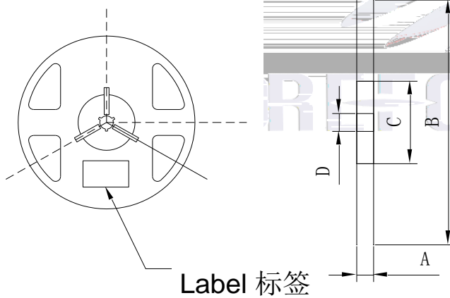
Fig.2-2 Reel Dimension
