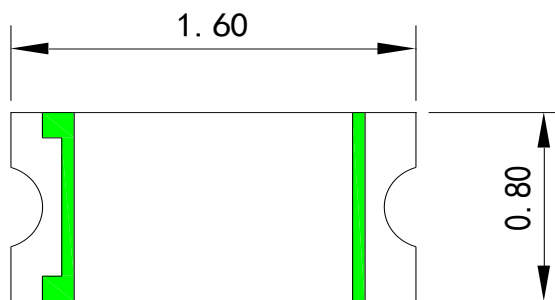
Fig.1-1 Top view
