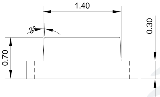
Fig.1-3 Side view
