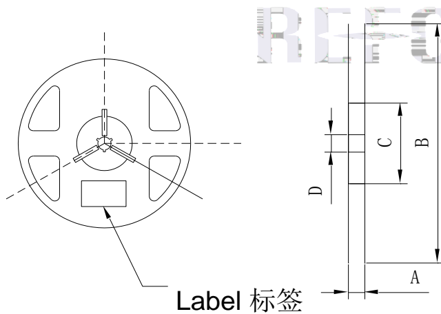
Fig.2-2 Reel Dimension
