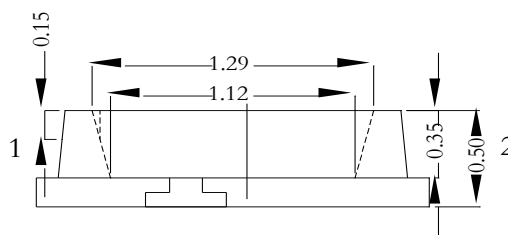
Fig.1-2 Side view
