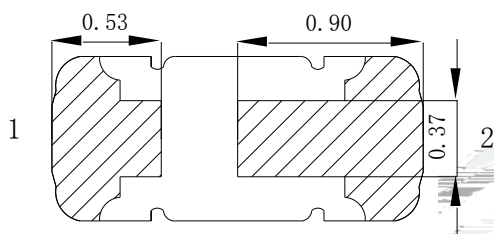
Fig.1-3 Bottom view
