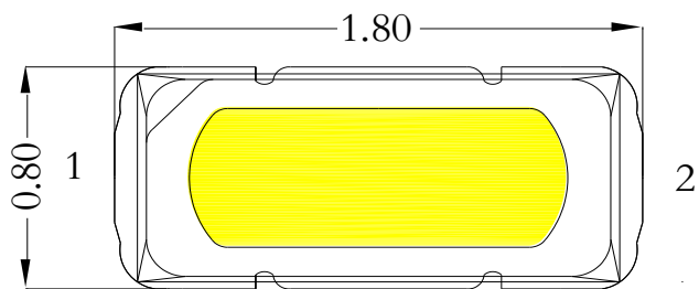
Fig.1-1 Top view
