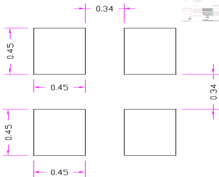
Fig.1-5 Soldering patterns
