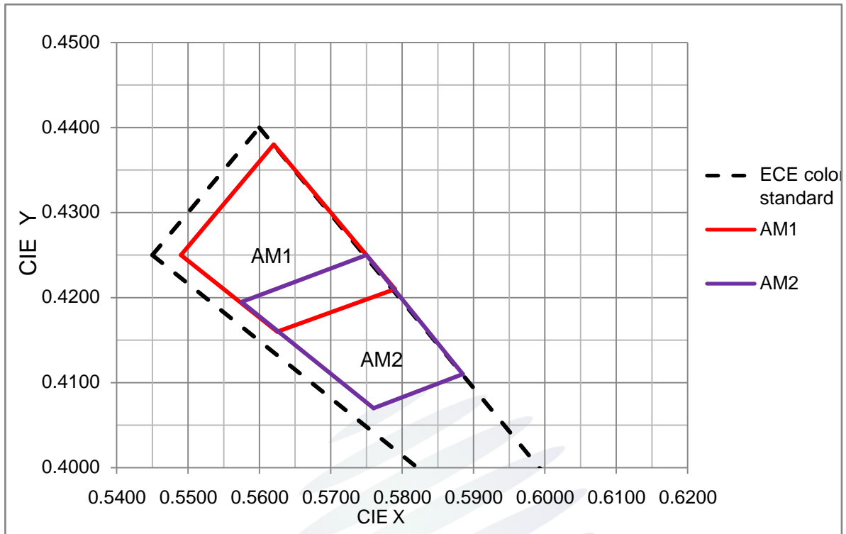
Fig. 1-6 The C.I.E Chromaticity Diagram CIE
