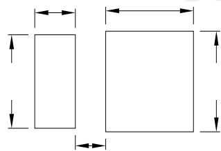
Fig.1-5 Soldering Patterns
