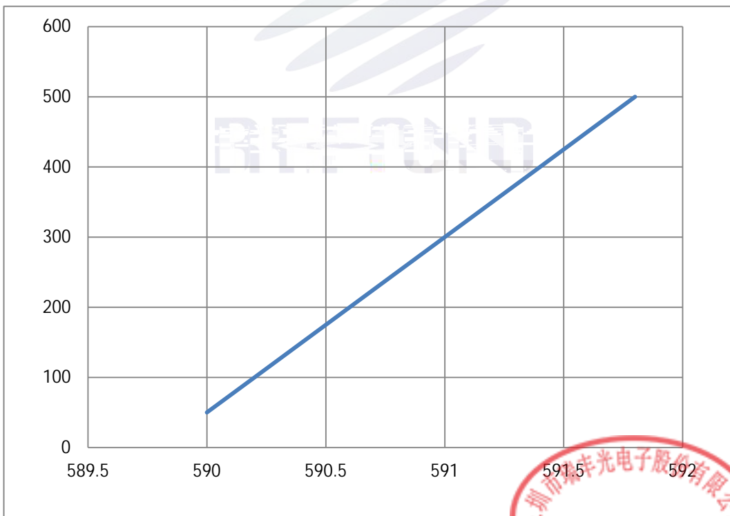
Fig. 1-12 Forward current vs. Color Shift
