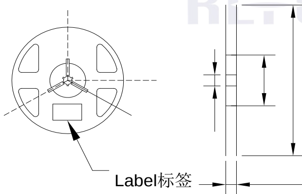
Fig.2-2 Reel Dimension
