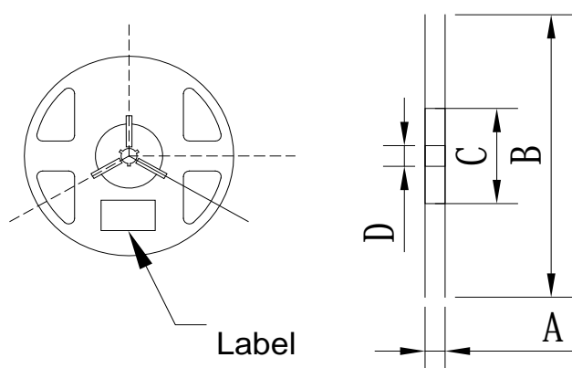
Fig.2-2 Reel Dimension
