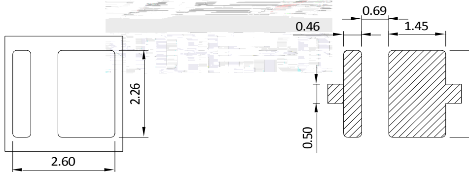
Fig.1-4 Bottom view
